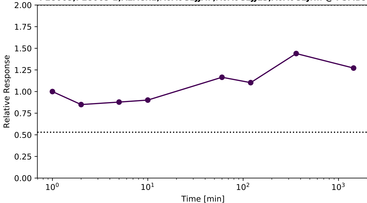
P28065;P28065-2;A2ACR1;A0A0G2JJA7;A0A0G2JJ13;A0A0G2JH.. @ PSMB9
