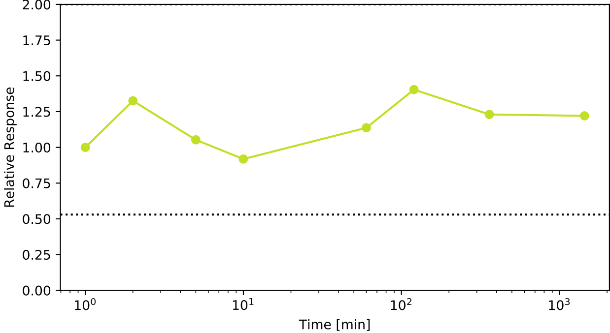
Q8IY22;A0A087WY48;Q8IY22-3;Q8IY22-2;A0A087WU05;A0A087.. @ CMIP
