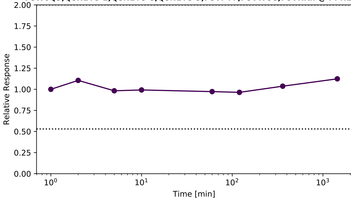
F8W0Q9;Q8NEY8-2;Q8NEY8-8;Q8NEY8-9;F8VPY7;F8VWU8;F8VRK.. @ PPHLN1
