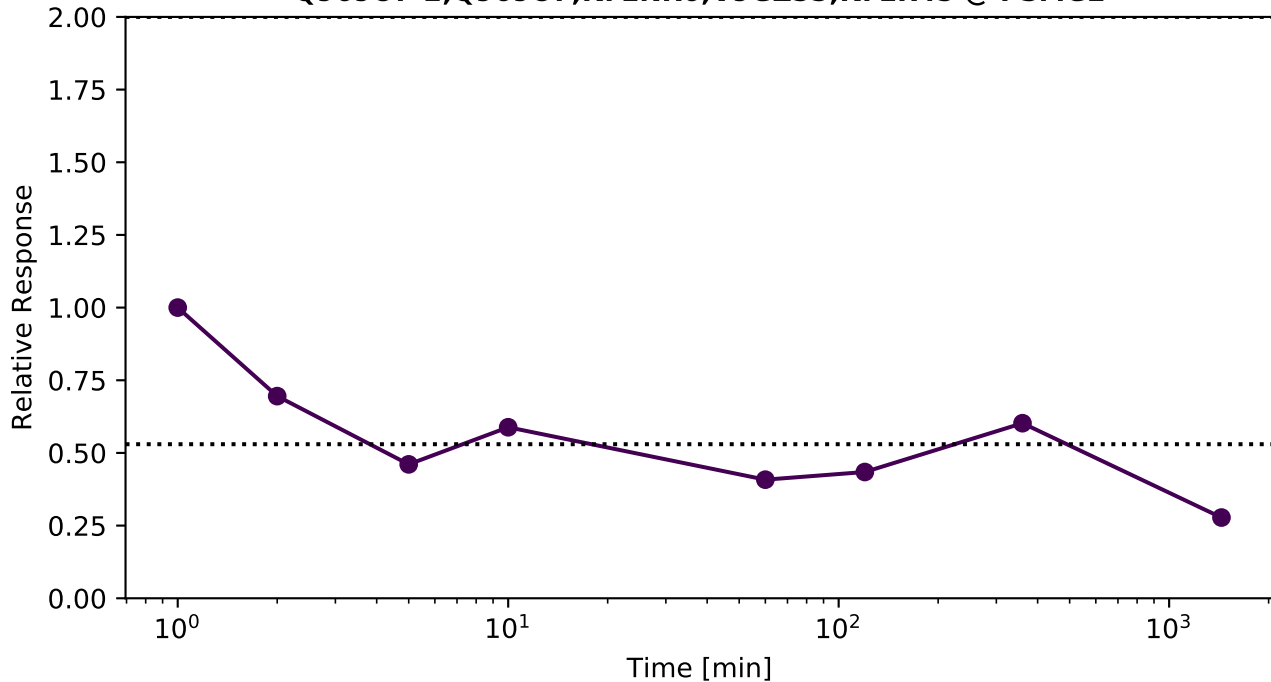
Q969U7-2;Q969U7;K7ENR6;V9GZ55;K7ER45 @ PSMG2
