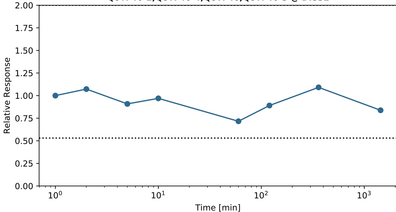
Q8TF46-2;Q8TF46-4;Q8TF46;Q8TF46-3 @ DIS3L
