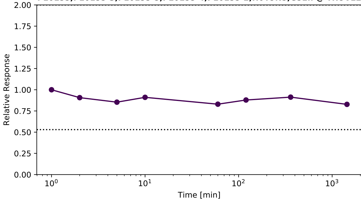
P10155;P10155-3;P10155-5;P10155-4;P10155-2;H0Y9N5;G5E.. @ TROVE2
