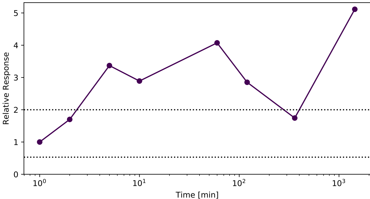
P22570-3;P22570;P22570-5;P22570-7;P22570-4;P22570-2;A.. @ FDXR
